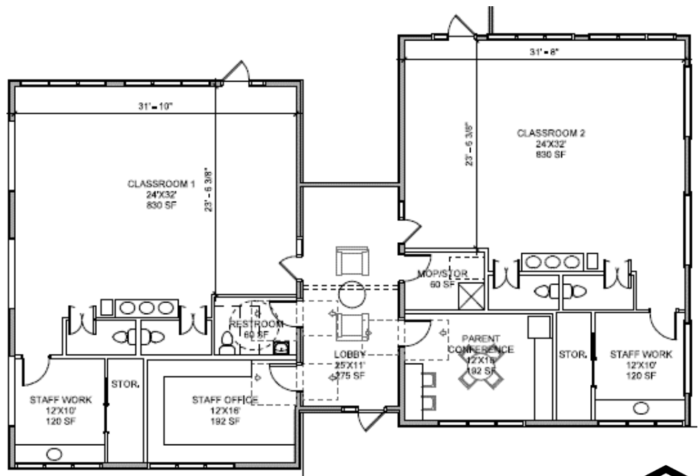
Top: Floor 3, lower level of Habitat homes Above: Floor 2, upper level of Habitat homes Right: spaces for Head Start classrooms
