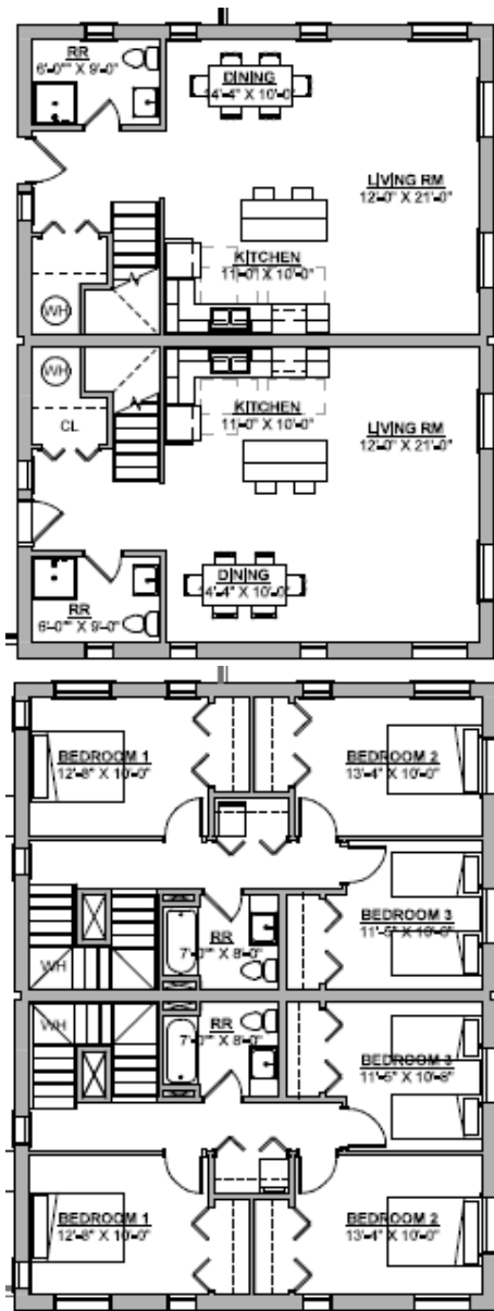
Top: Floor 3, lower level of Habitat homes Above: Floor 2, upper level of Habitat homes Right: spaces for Head Start classrooms
